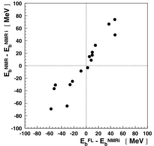
Fig. 10. For each NMR probe, the difference between the FL energy, from method B, and that estimated from the NMR probe is plotted against the difference between the mean NMR energy, averaged over all probes, and that from the individual probe in physics running. The differences are calculated at a beam energy of 100 GeV
