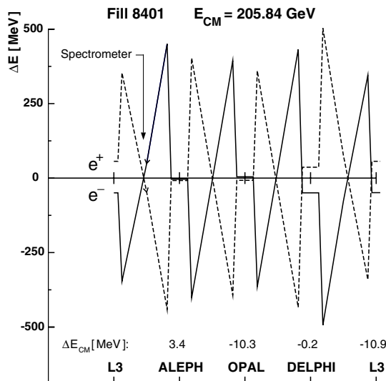
Fig. 7. The RF sawtooth for a typical RF configuration in 2000. The electron beam is represented by the left-going solid line, the positron beam by the right-going dotted line. The locations of the experiments and the LEP spectrometer are indicated. \Delta E = 0 corresponds to the average beam energy of LEP. \Delta E_{CM} is the correction to E_{CM}^{MOD} at each IP due to RF effects
