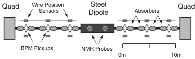
Fig. 15. A schematic of the LEP spectrometer, situated between two quadrupole magnets close to IP3. The various components are discussed in the text
