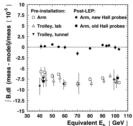
Fig. 18. Relative residuals from the dipole magnet mapping campaigns, plotted against energy. Results are shown for all the mapping configurations discussed in the text. In all cases the model derives from a fit to the 'Post-LEP: Arm, new Hall probes' data. The horizontal positions of certain points have been slightly adjusted to aid clarity
