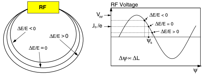
Fig. 37. Change of orbit length ( \Delta L ) for particles with energy deviation ( \Delta E ) in an accelerator with a single RF cavity (left). Accelerating voltage as a function of phase; particles with different energies arrive at different phases, thus seeing a voltage different from that needed to compensate the nominal energy loss per turn (right)
