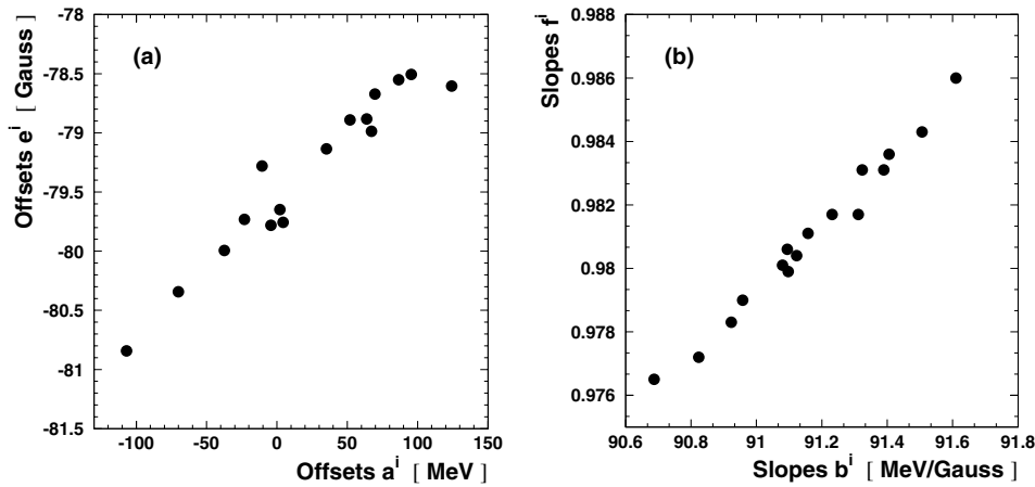
Fig. 9. The offsets a and slopes b of (5) and 15 comparing the field measured by each NMR probe with the RDP and FL measurements. The values shown are averages over all the FL measurements. There is one entry per NMR probe in each plot
