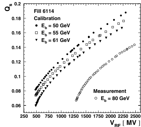
Fig. 39. Measured Q_s is shown against V_{RF} for different beam energies. The calibration set for the voltage calibration factor is indicated, together with the high-energy data
