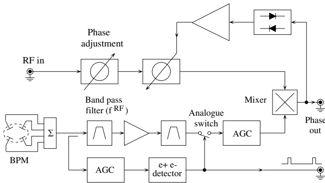
Fig. 38. A schematic block diagram of the LEP synchrotron oscillation detector
