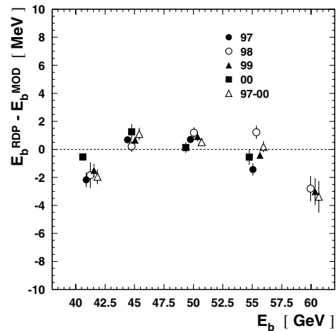
Fig. 2. Residuals of the fitted energy model to the RDP data in 1997–2000. Each point is the mean over the available measurements at that energy, with the error bar the statistical uncertainty on this mean. The horizontal positions of the points have been slightly adjusted to aid clarity
