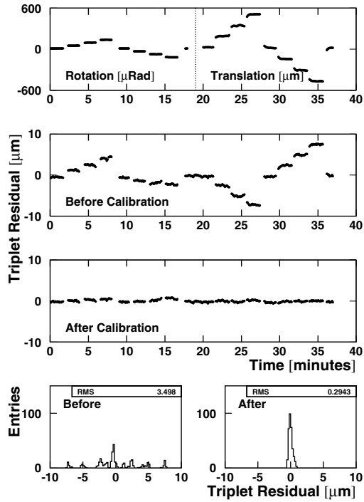
Fig. 23. BPM relative-gain calibration. Displayed, as a function of time, are the beam movements in the calibration procedure, and the triplet residual before and after calibration. Also shown are the projections of the triplet residuals
