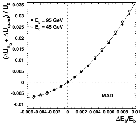
Fig. 41. Variation of relative energy loss with relative energy change induced by beam offsets in the quadrupoles. The results are calculated with MAD for two energy points. A common parameterisation is superimposed. Note that during operation the relative energy change from beam offsets is typically \leq 10^{-4}
