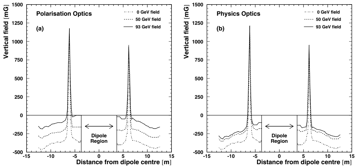
Fig. 19. Environmental magnetic field readings in the vertical direction as a function of longitudinal position along the spectrometer for the polarisation a and physics b optics. The dipole region is not shown. The large spikes are caused by permanent magnets situated in vacuum pumps
