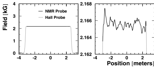
Fig. 17. The longitudinal profile of the spectrometer dipole field at an excitation current corresponding to 100 GeV as measured by the mapping campaigns. Also shown is a zoom of the core region for a single map
