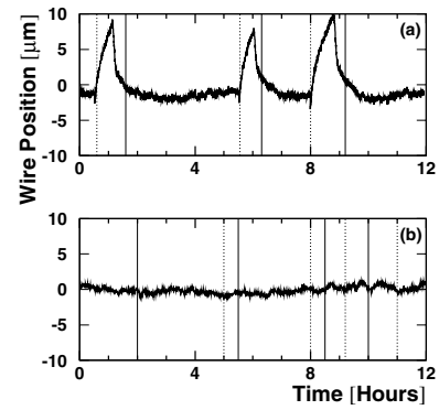
Fig. 25. The response of a reference WPS over two 12-hour periods before a and after b additional radiation shielding was installed, and the wire centred within the sensor. The vertical solid lines indicate the declared start-of-fill and the dotted lines indicate a beam dump. Note that b encompasses fills in which actual spectrometer measurements were performed
