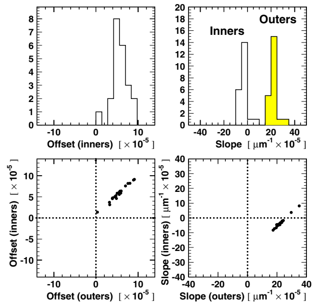
Fig. 34. Variations in the fit result for the offset and the slopes for the inner and outer BPM combinations from various combinations of fills in the low-energy sample. Each entry corresponds to a distinct subset, varying in size between 4 and 13 energy points
