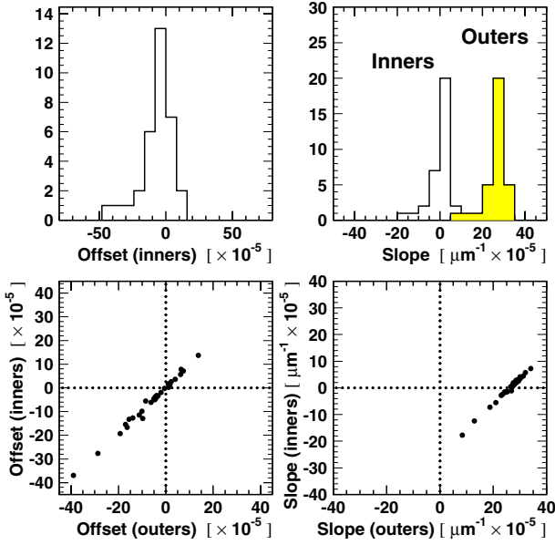
Fig. 32. Variations in the fit result for the offset and the slopes for the inner and outer BPM combinations calculated from various combinations of fills in the high-energy sample. Each entry corresponds to a distinct subset, varying in size between 7 and 17 fills
