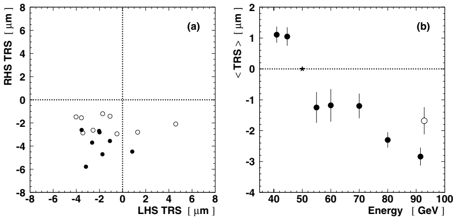
Fig. 28. Characteristics of the triplet-residual shifts: a shows the TRS in the left and right arms for the high-energy sample; b shows the mean TRS averaged over both arms ( \langle \text{TRS} \rangle ), referenced to 50 GeV (asterisk), as a function of energy, for the full multi-point dataset. The full points represent the polarisation optics and the open points the physics optics
