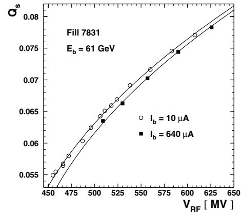
Fig. 42. Q_s as function of total RF voltage for two different bunch currents in fill 7831, showing the effect of the parasitic mode losses. The curves are individual fits to each dataset
