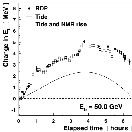
Fig. 5. Comparison between the tide and NMR rise components of the energy model and RDP measurements for fill 6432. The tide contribution is also shown separately
