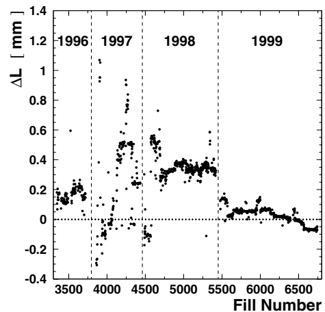
Fig. 6. The orbit lengthening \Delta L caused by the horizontal correctors, plotted against fill number for 1996–1999
