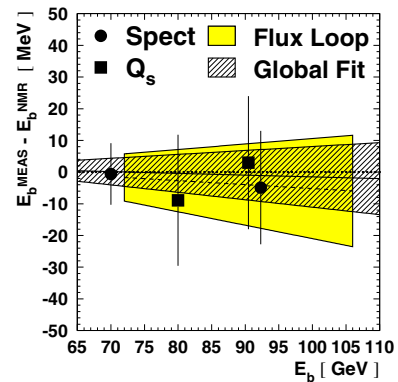
Fig. 45. The difference between the measurements of E_b and the NMR model prediction, together with the results of the two-parameter fit. In the fit, the Q_s data consist of five measurements at E_b = 80 GeV and one more precise measurement at E_b = 90 GeV. The 80 GeV measurements have been combined into a single point in this figure. Measurements made with the same method have correlations which are discussed in the text
