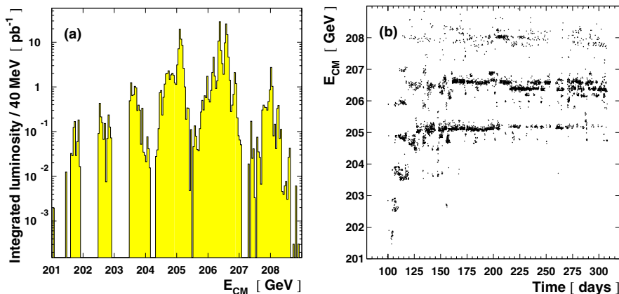
Fig. 1. Distributions of collected luminosity for a single LEP experiment in 2000. a shows the integrated luminosity in bins of E_{\text{CM}} . b shows the variation of E_{\text{CM}} against day of year; each entry corresponds to the mean energy for a data file of maximum length \sim 30 minutes. The values of E_{\text{CM}} have been calculated using the full energy model
