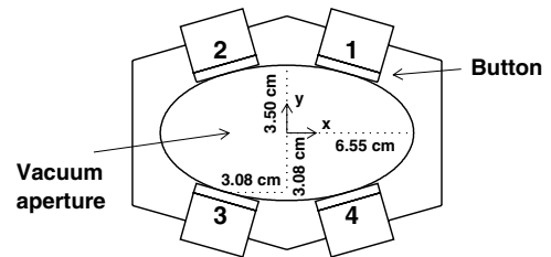
Fig. 21. Schematic of a LEP BPM-block and its button sensors, indicating the dimensions and the button numbering convention assumed in the text
