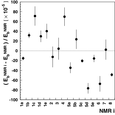
Fig. 3. Relative differences between the individual probe predictions of the dipole energy and that of the average, evaluated at physics energy and averaged over 1997–2000. The error bars are half the difference between the maximum and minimum values in these years
