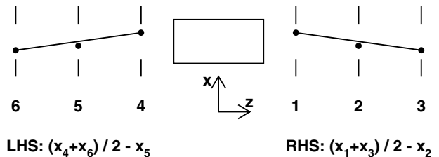
Fig. 22. The definition of the BPM numbering scheme and bending plane triplet residuals
