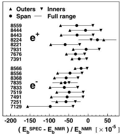
Fig. 29. Spectrometer results compared with the NMR model at high energy. For each measurement a spread is indicated showing the variation coming from the choice of 9 possible BPM combinations (‘Full range’), of which 3 specific cases are indicated (‘Outers’, ‘Inners’ and ‘Span’, defined as in Fig. 30)
