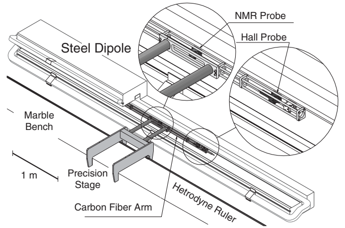
Fig. 16. The magnetic mapping test stand, showing inset the components of the moving arm
