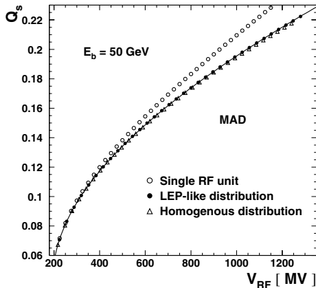
Fig. 40. Synchrotron tune as a function of total RF voltage as calculated with the MAD program for different RF configurations. The curve is a fit to the correct RF distribution using the model of (26)
