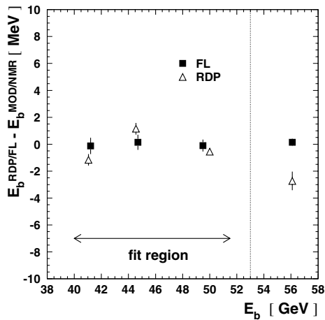
Fig. 14. Residuals from the NMR fits to the RDP data and FL data for all years, using method A. The error bars indicate the statistical scatter over the measurements. Only the data below 55 GeV are used in the fits. (Note also that the RDP data at 55 GeV and 60 GeV, plotted separately in Fig. 2, have here been averaged together into a single point)
