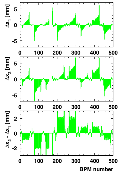
Fig. 8. An example of the difference between electron and positron orbits ( \Delta x_i vs. BPM number) for two different RF configurations (configuration 1 top; configuration 2 middle). IPs 2,4,6 and 8 are situated close to BPMs 60, 190, 310 and 440 respectively. The energy sawtooth is clearly visible. The difference of the two orbit differences is displayed on the bottom plot. The step changes reflect the different energy gains at the four IPs for the two configurations. Note that the orbit information is missing between BPMs 160 and 176
