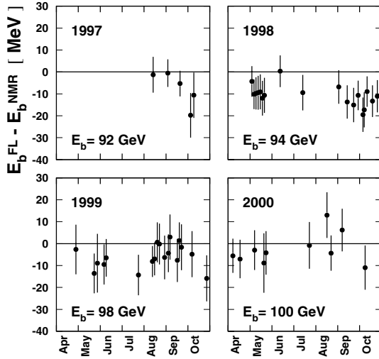
Fig. 12. The difference, in MeV, between the magnetic field measured by the FL and predicted by the NMR probes for each of the FL measurements, using method B. The data are shown separately for each year
