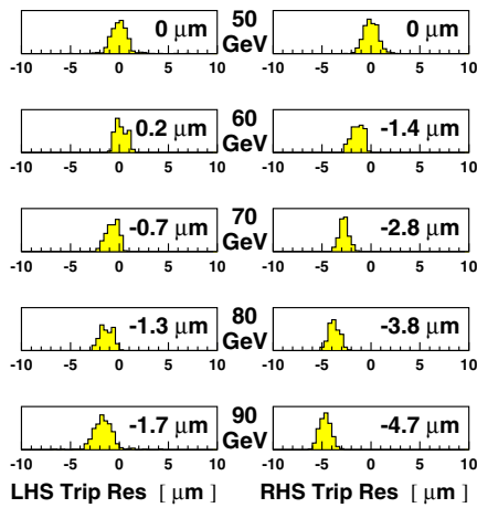
Fig. 27. BPM triplet residuals for fill 8443. The gains have been calibrated and the triplet residuals centred at 50 GeV. Good resolution is observed at the other energy points, but accompanied by residual shifts. The inset numbers indicate the means of the distributions
