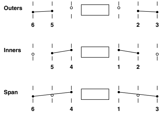
Fig. 30. A schematic illustrating the three choices of BPM combinations used for determining the bending angle in the spectrometer energy analysis
