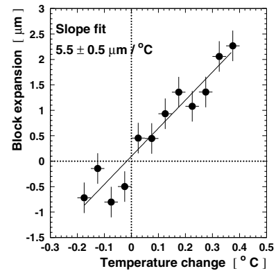
Fig. 26. BPM-block expansion as measured by the WPS system against temperature change during spectrometer measurements. The data are averaged over all six stations. A linear fit is superimposed
