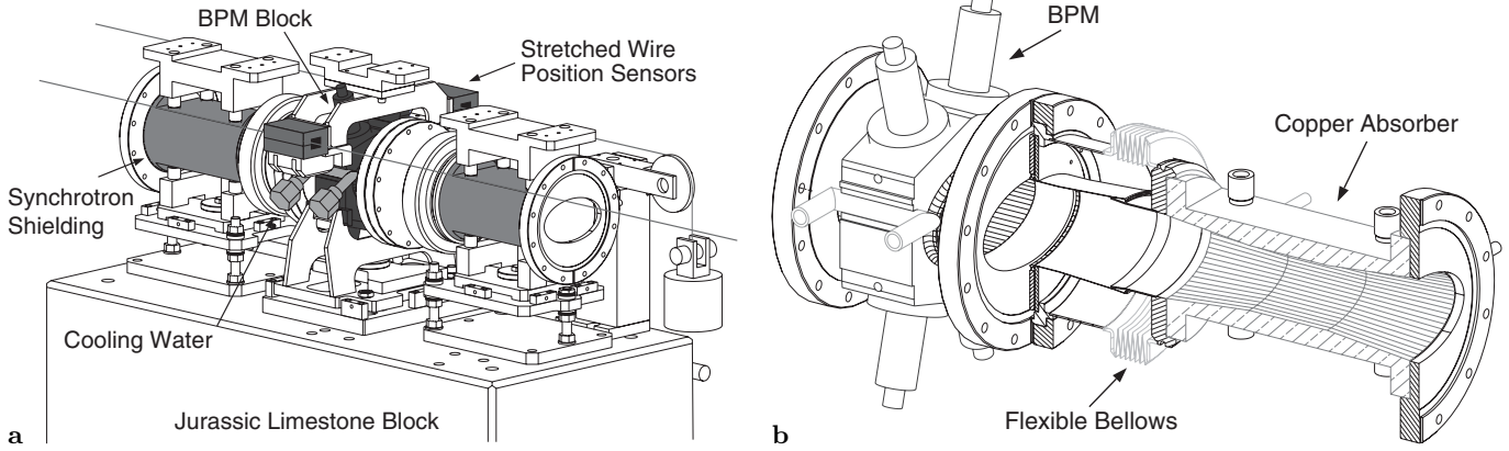
Fig. 20. A spectrometer BPM station a , and a cut away view of the BPM block and absorber b . The various components are discussed in the text
