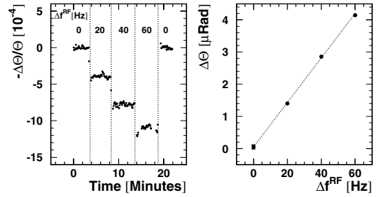
Fig. 24. The change of bending angle measured in the spectrometer as the energy is varied through a manipulation of the RF frequency. The dependence is linear with a slope value consistent with expectations
