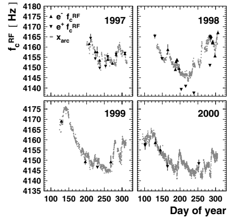
Fig. 4. Evolution of the central frequency as a function of time for the four main datasets of the LEP 2 programme. Shown are both the actual f_c^{\text{RF}} measurements, and the values extracted from x_{\text{arc}} , after correction for tides. Note that the vertical scale shows a variation in the last four digits of the LEP RF frequency, which is nominally 352 254 170 Hz
